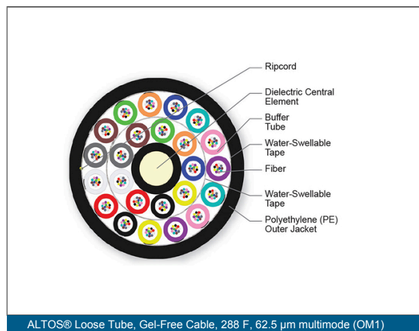
ALTOS® Loose Tube, Gel-Free Cable, 288 F, 62.5 \mu m multimode (OM1)
